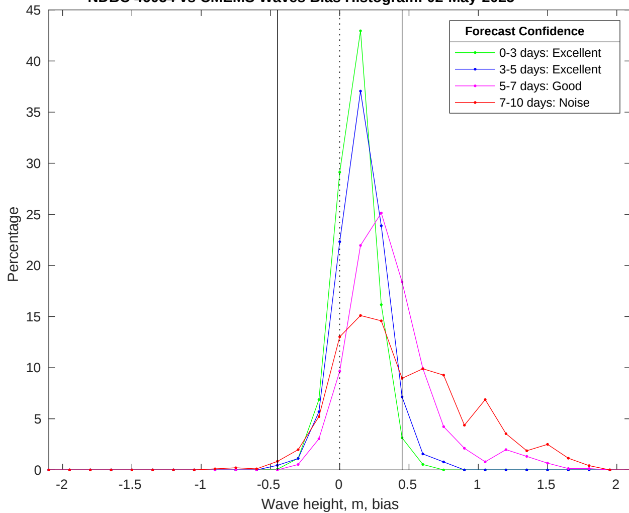
NDBC 46054 vs CMEMS Waves Bias Histogram: 02-May-2025
