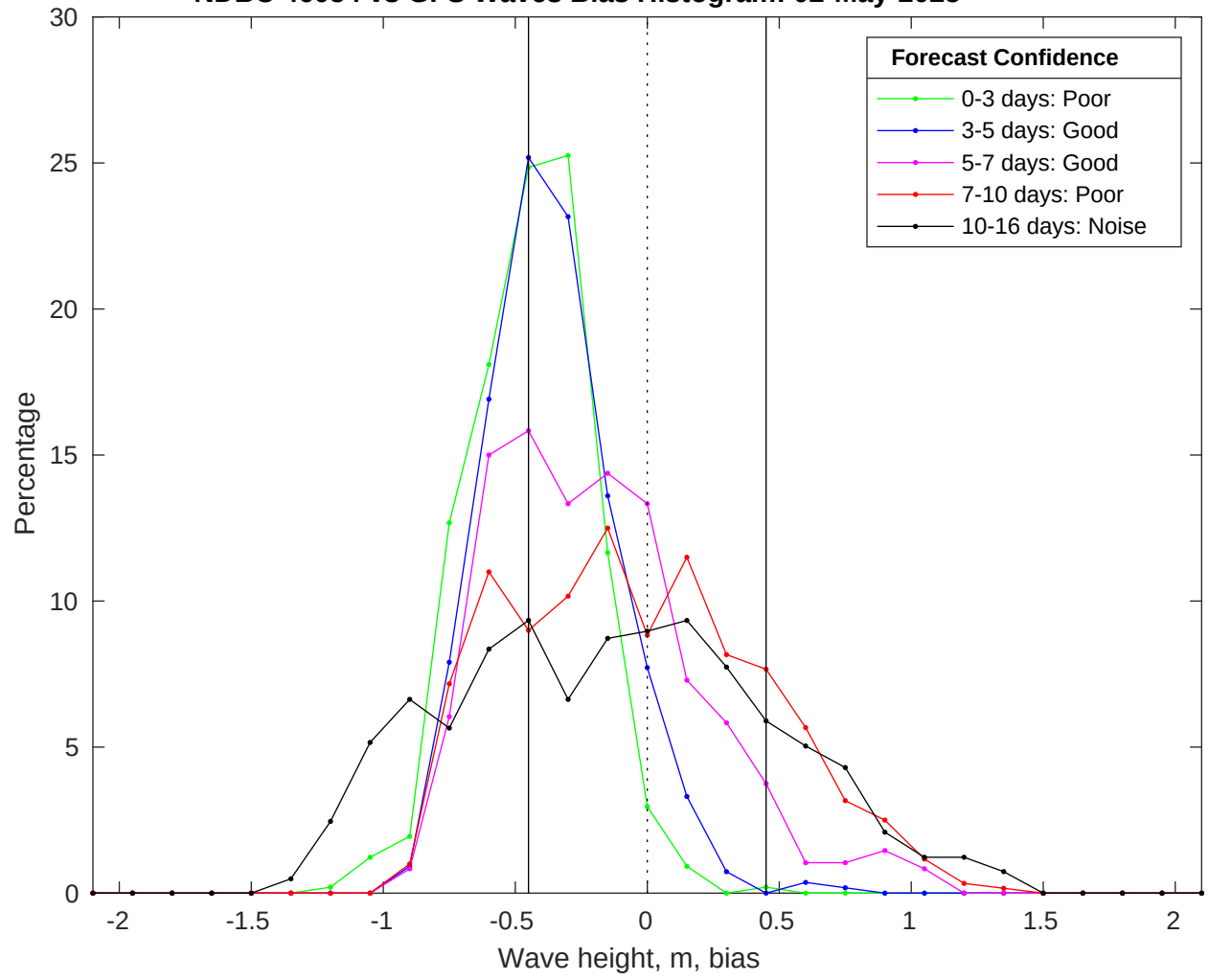
NDBC 46054 vs GFS Waves Bias Histogram: 02-May-2025
