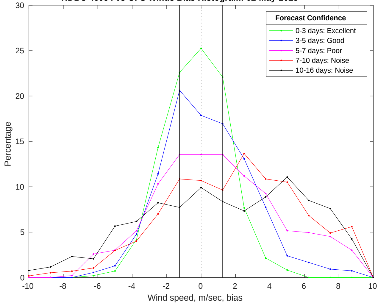
NDBC 46054 vs GFS Winds Bias Histogram: 02-May-2025
