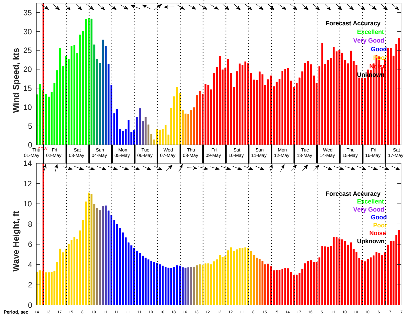
Wind & Wave Forecast for NDBC 46054 from 01-May-2025 16:00:00 to 17-May-2025 16:00:00
