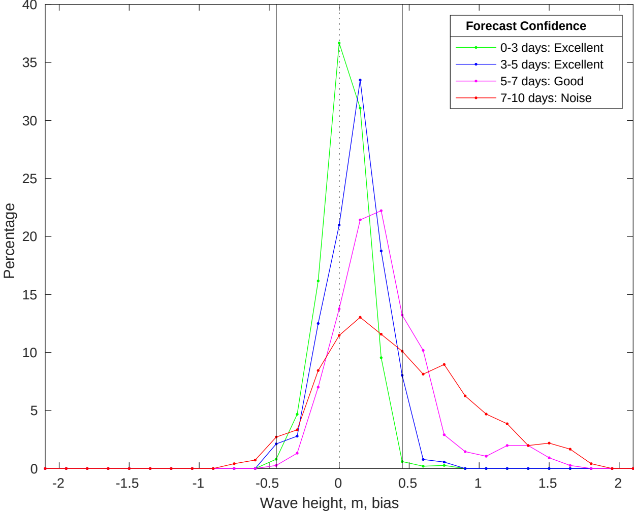
NDBC 46069 vs CMEMS Waves Bias Histogram: 02-May-2025
