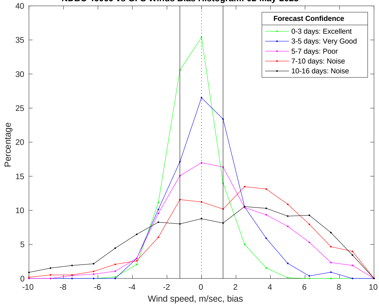
NDBC 46069 vs GFS Winds Bias Histogram: 02-May-2025
