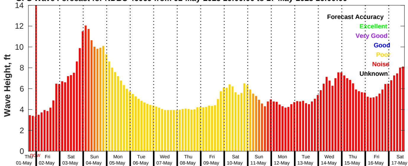
GFS Wave Forecast for NDBC 46069 from 01-May-2025 16:00:00 to 17-May-2025 16:00:00
