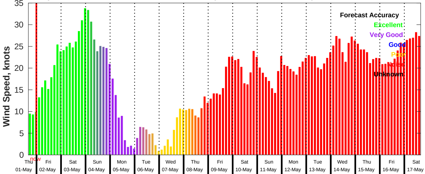
GFS Wind Speed Forecast for NDBC 46069 from 01-May-2025 16:00:00 to 17-May-2025 16:00:00
