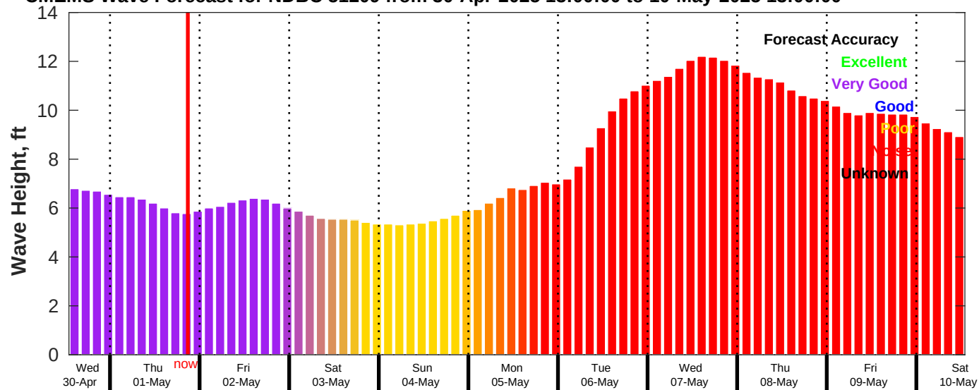
CMEMS Wave Forecast for NDBC 51209 from 30-Apr-2025 13:00:00 to 10-May-2025 13:00:00
