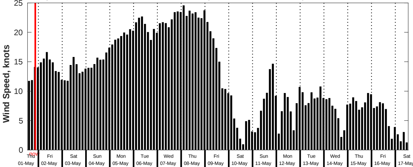
GFS Wind Speed Forecast for NDBC 51209 from 01-May-2025 13:00:00 to 17-May-2025 13:00:00
