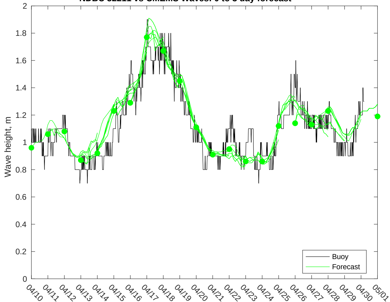
NDBC 52211 vs CMEMS Waves: 0 to 3 day forecast
