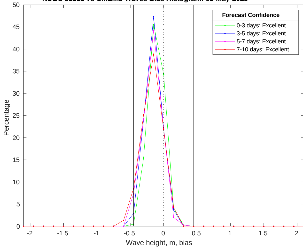
NDBC 52212 vs CMEMS Waves Bias Histogram: 02-May-2025
