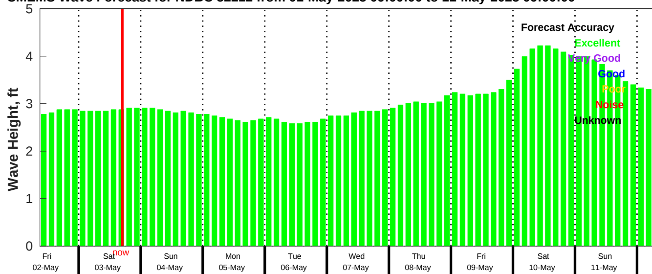
CMEMS Wave Forecast for NDBC 52212 from 01-May-2025 09:00:00 to 11-May-2025 09:00:00
