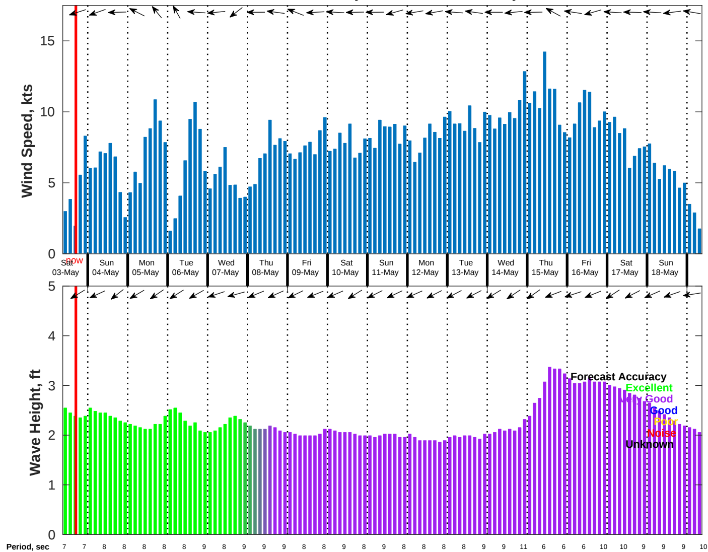
Wind & Wave Forecast for NDBC 52212 from 02-May-2025 09:00:00 to 18-May-2025 09:00:00
