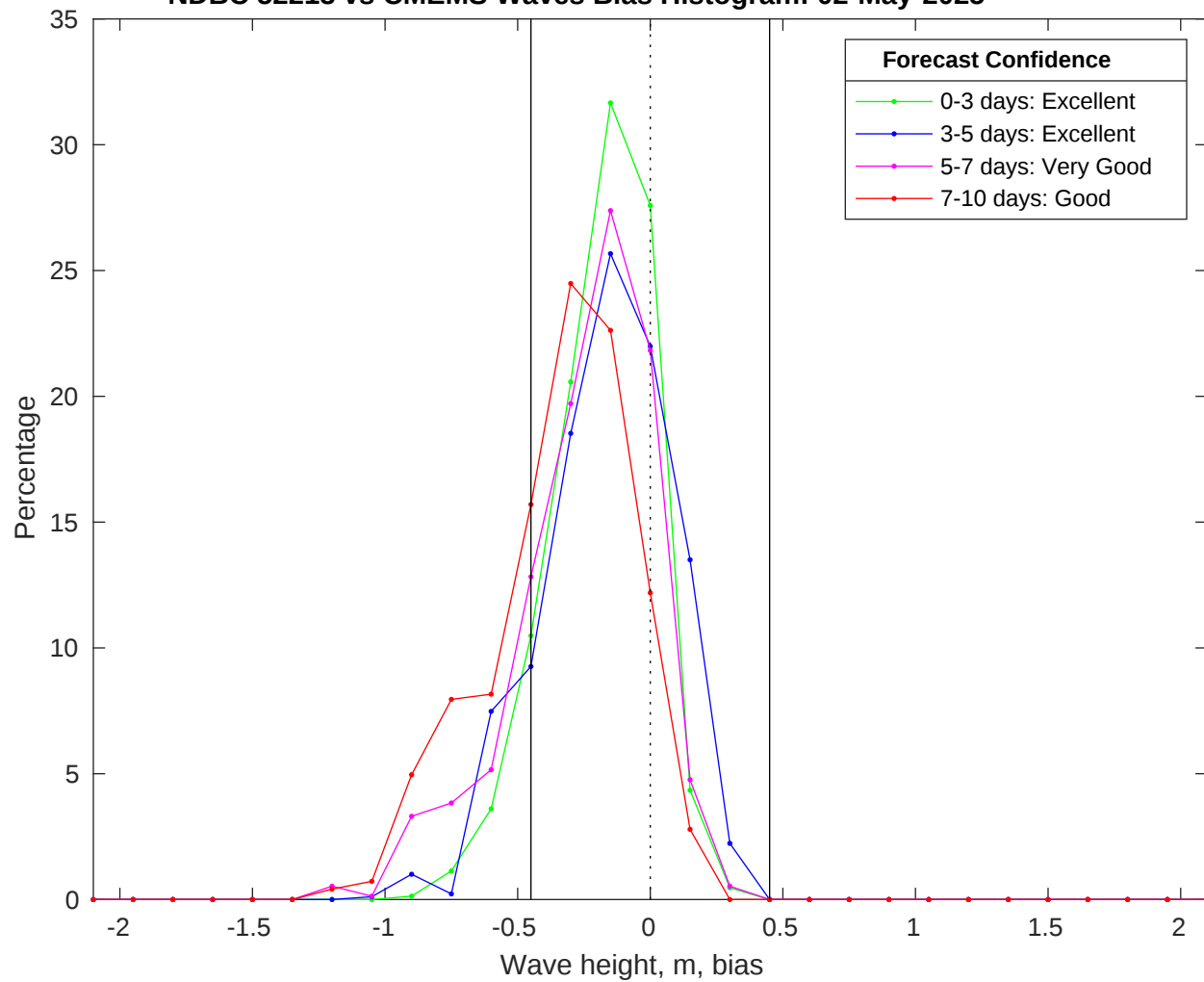
NDBC 52213 vs CMEMS Waves Bias Histogram: 02-May-2025
