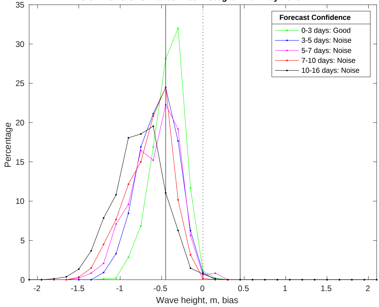
NDBC 52213 vs GFS Waves Bias Histogram: 02-May-2025
