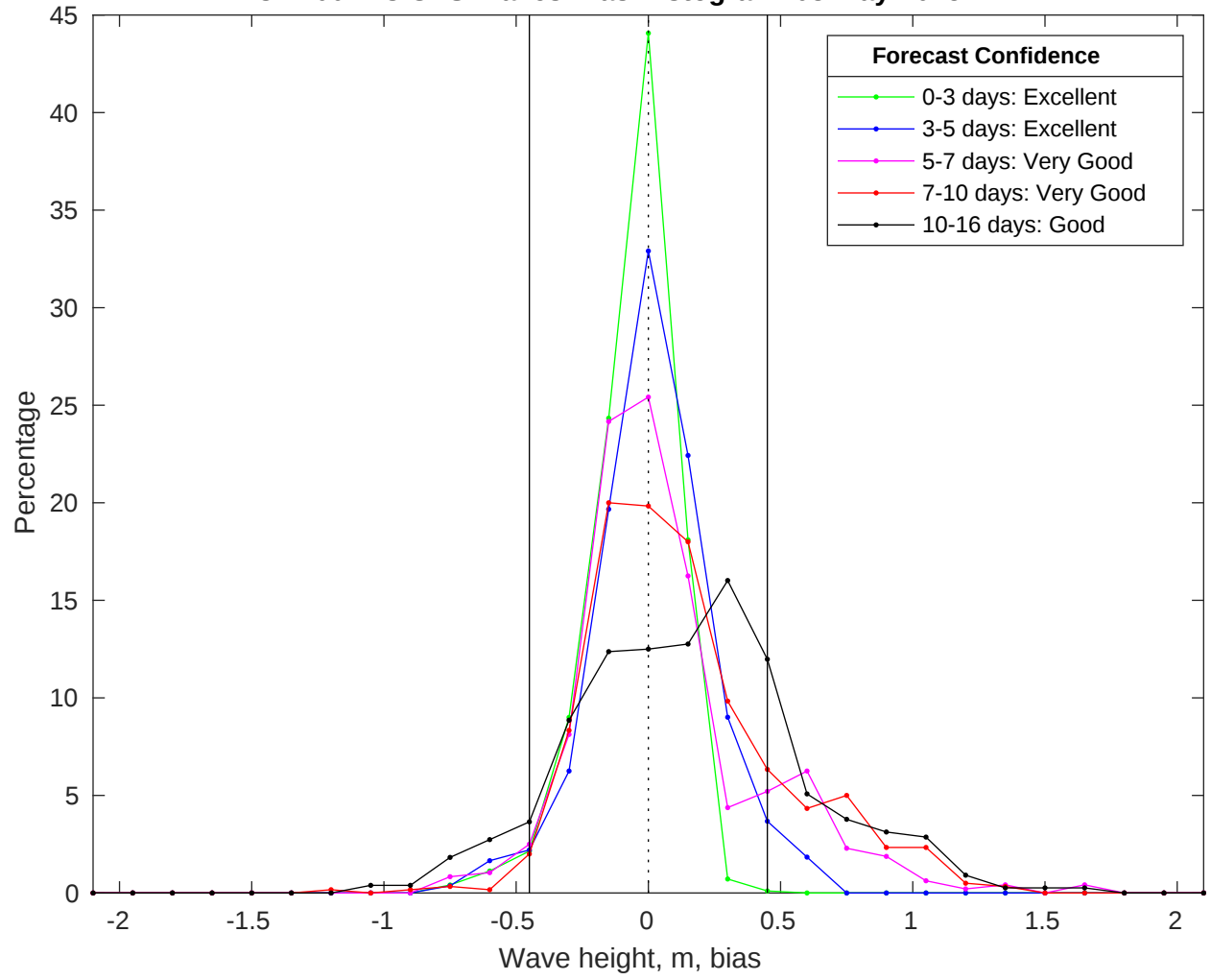
NDBC 41004 vs GFS Waves Bias Histogram: 03-May-2025
