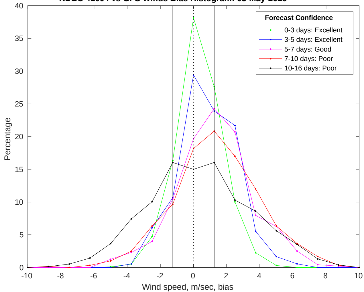
NDBC 41004 vs GFS Winds Bias Histogram: 03-May-2025
