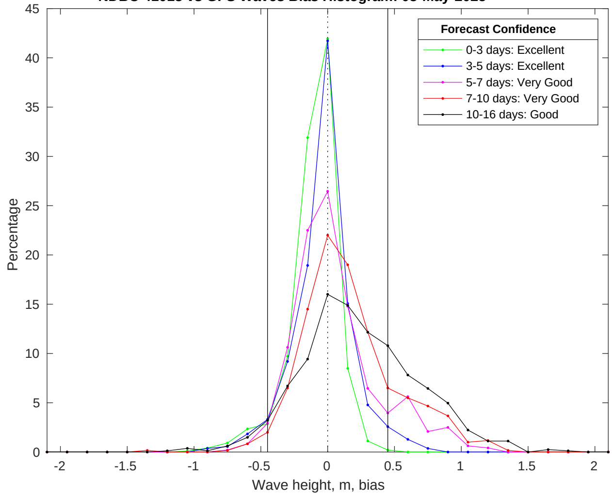
NDBC 41013 vs GFS Waves Bias Histogram: 03-May-2025
