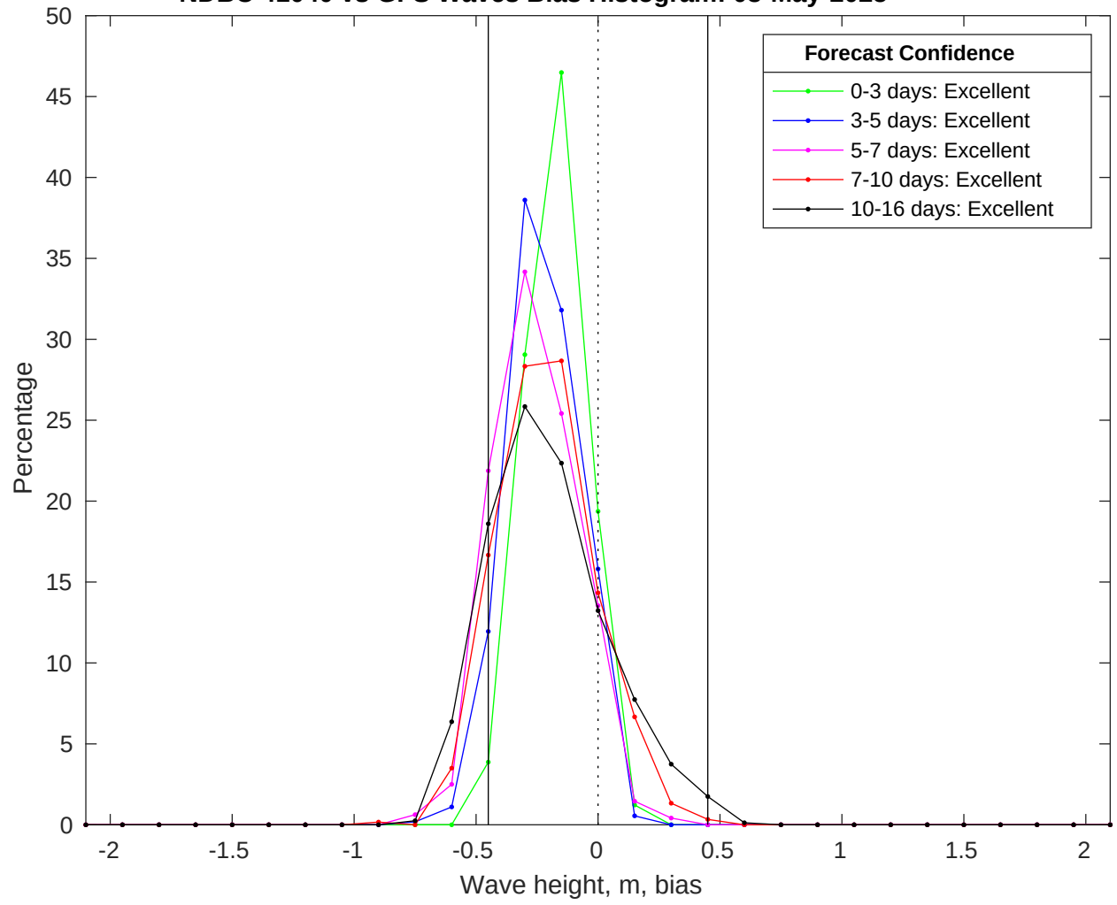
NDBC 41040 vs GFS Waves Bias Histogram: 03-May-2025
