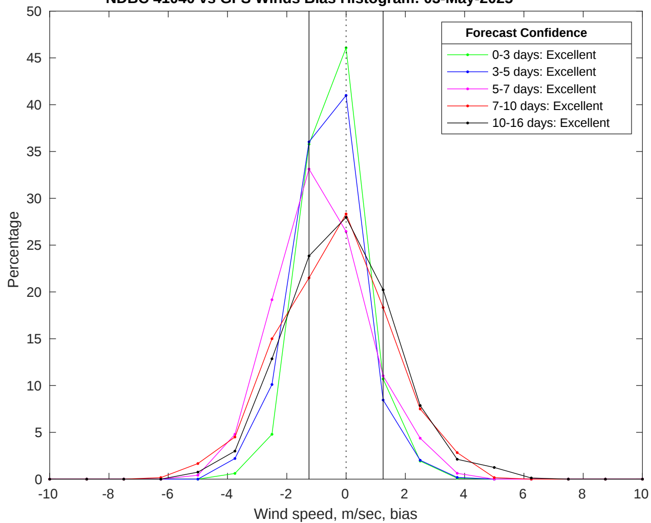
NDBC 41040 vs GFS Winds Bias Histogram: 03-May-2025
