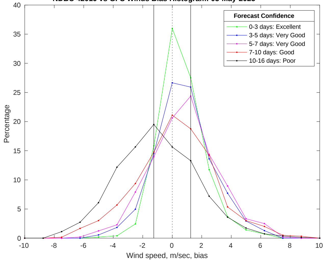
NDBC 42019 vs GFS Winds Bias Histogram: 03-May-2025
