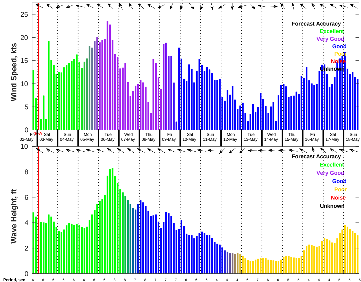
Wind & Wave Forecast for NDBC 42019 from 02-May-2025 18:00:00 to 18-May-2025 18:00:00
