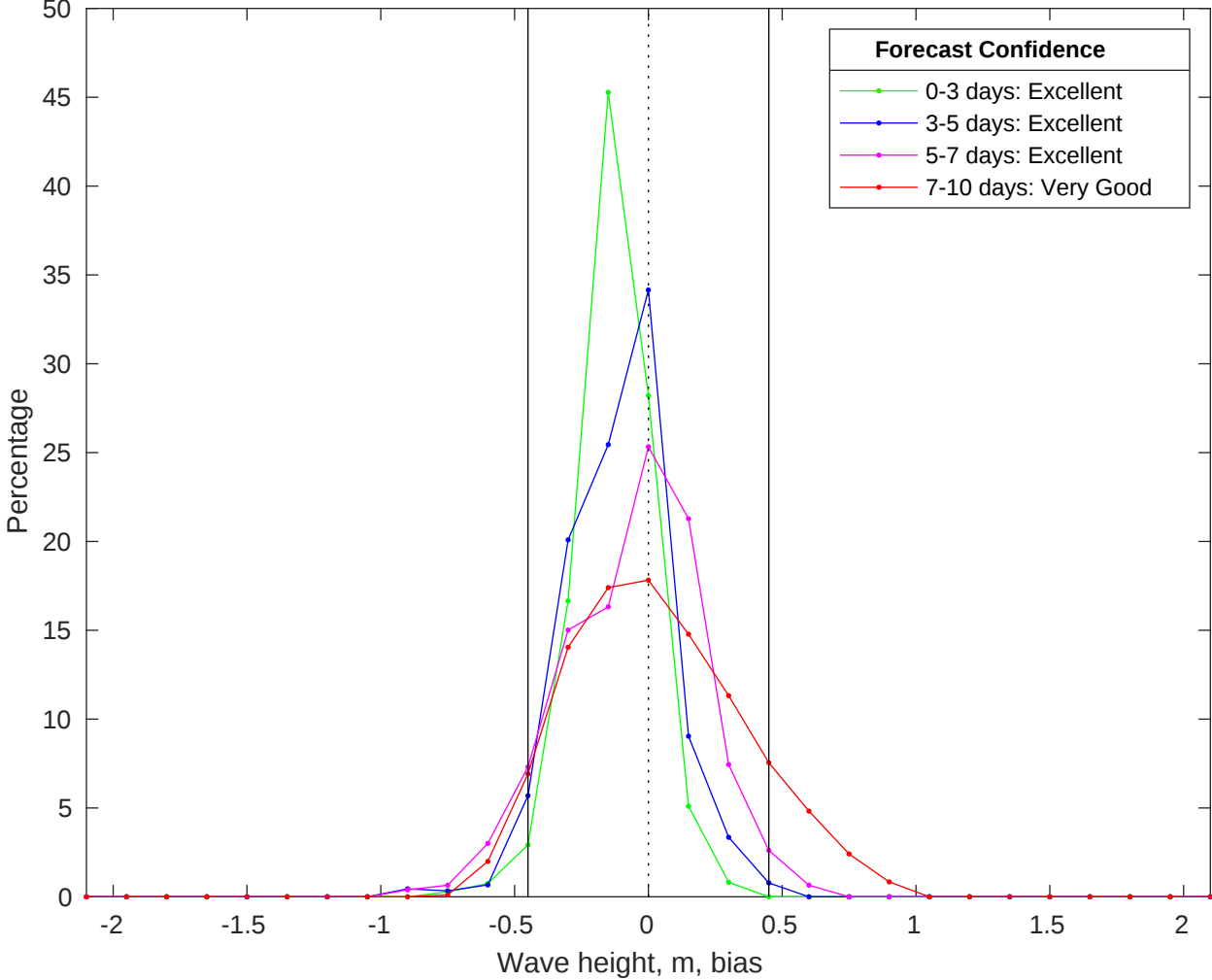
NDBC 42020 vs CMEMS Waves Bias Histogram: 03-May-2025
