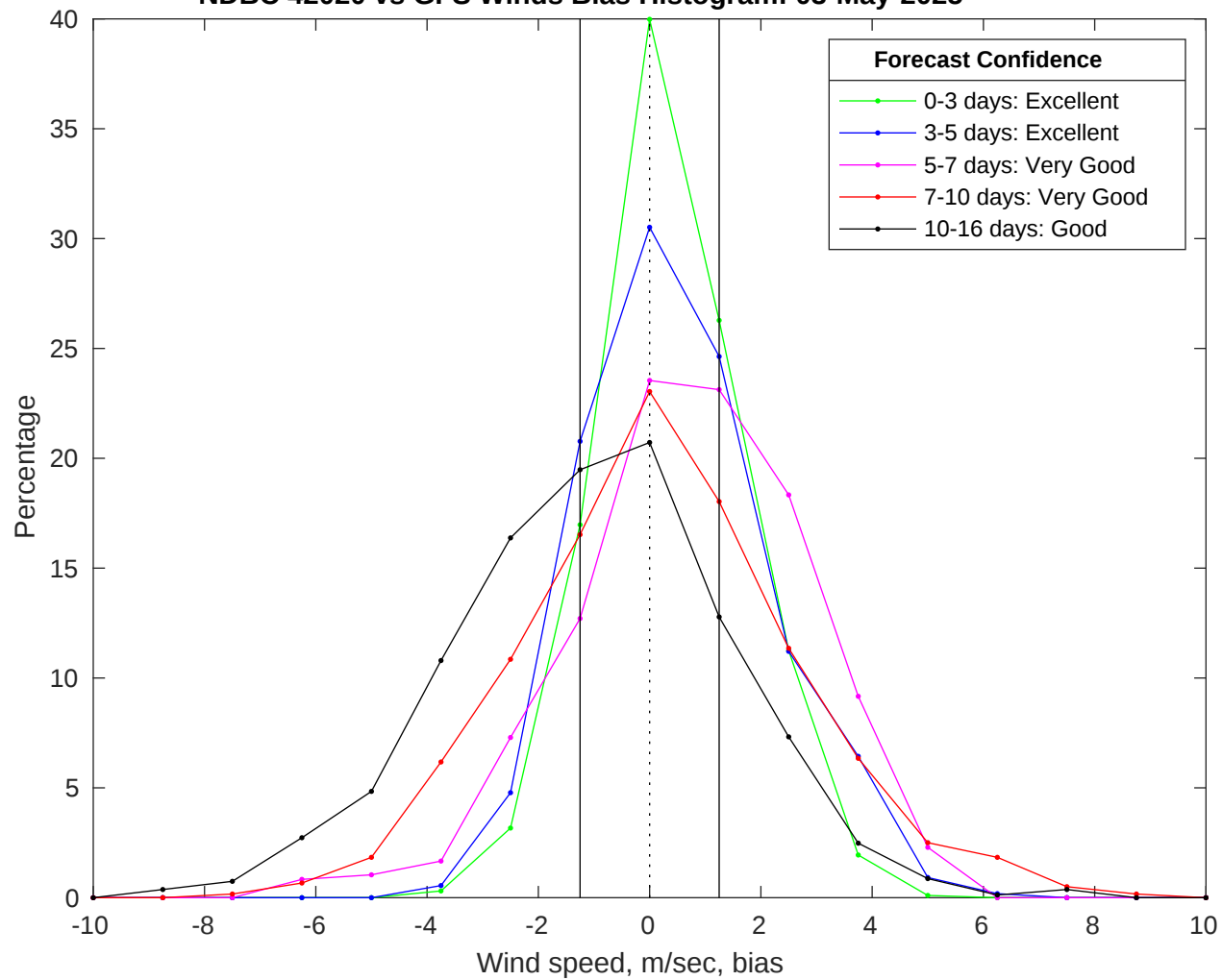
NDBC 42020 vs GFS Winds Bias Histogram: 03-May-2025
