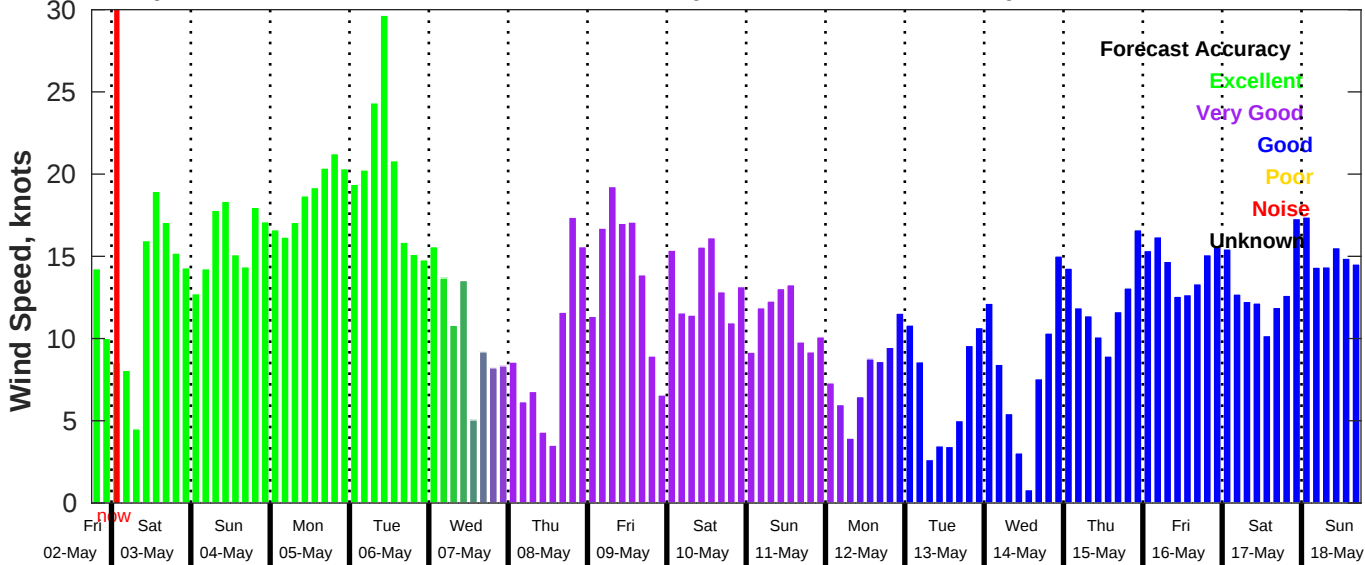
GFS Wind Speed Forecast for NDBC 42020 from 02-May-2025 18:00:00 to 18-May-2025 18:00:00
