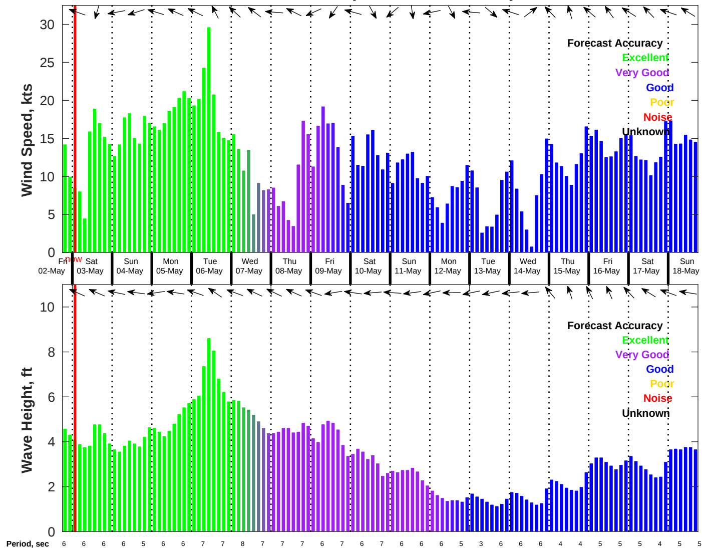
Wind & Wave Forecast for NDBC 42020 from 02-May-2025 18:00:00 to 18-May-2025 18:00:00
