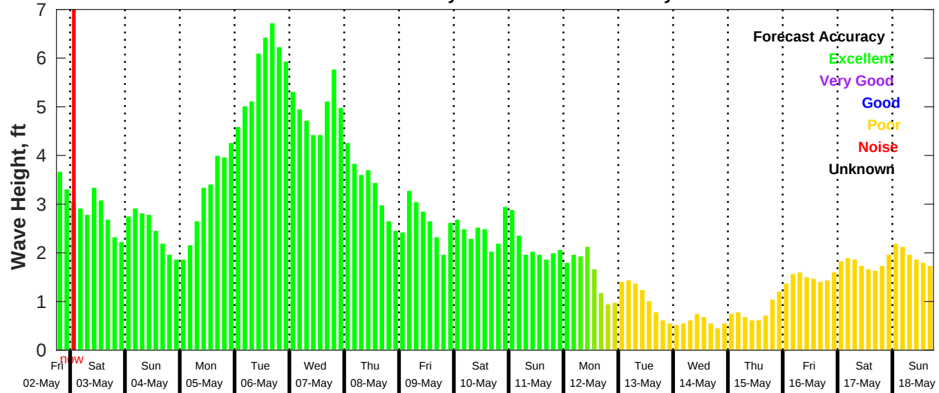
GFS Wave Forecast for NDBC 42035 from 02-May-2025 18:00:00 to 18-May-2025 18:00:00
