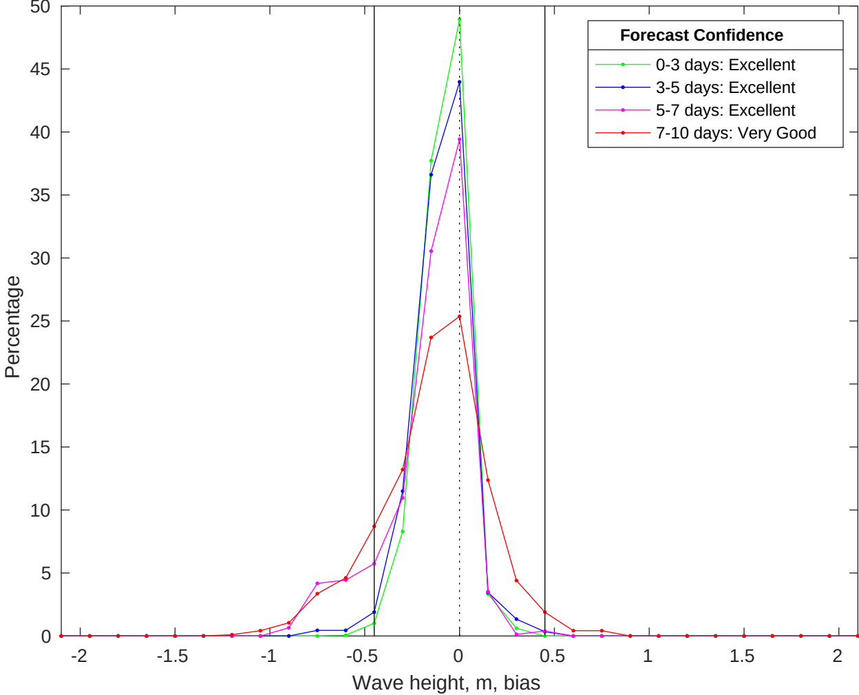
NDBC 42036 vs CMEMS Waves Bias Histogram: 03-May-2025
