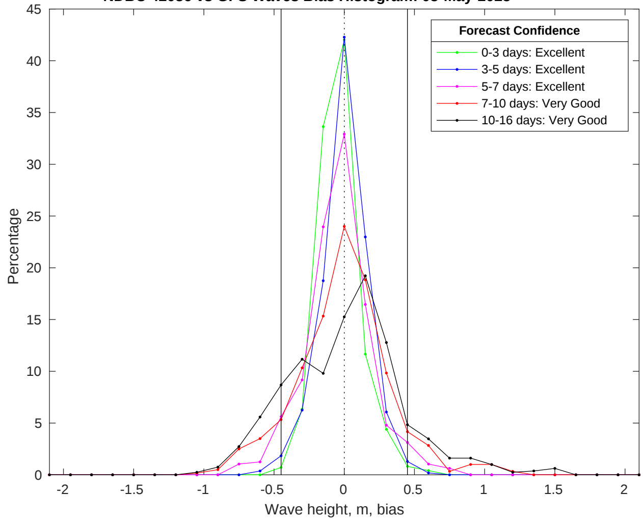
NDBC 42036 vs GFS Waves Bias Histogram: 03-May-2025
