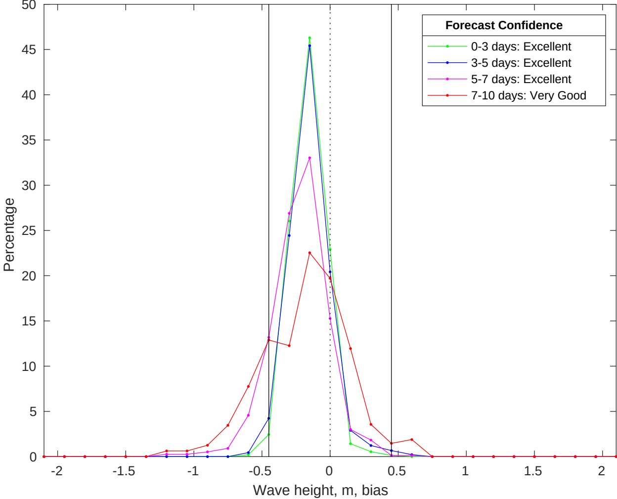
NDBC 42040 vs CMEMS Waves Bias Histogram: 03-May-2025
