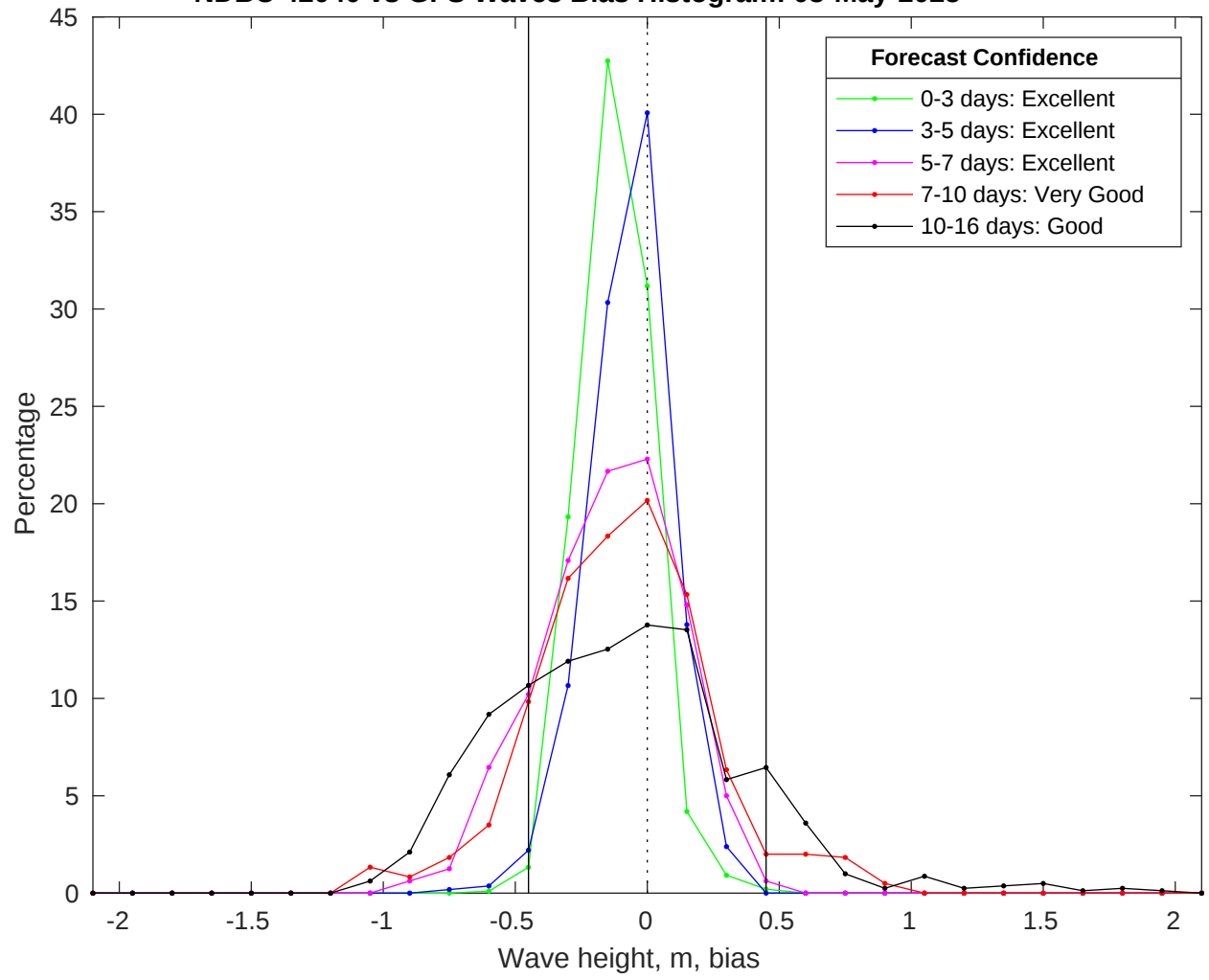
NDBC 42040 vs GFS Waves Bias Histogram: 03-May-2025
