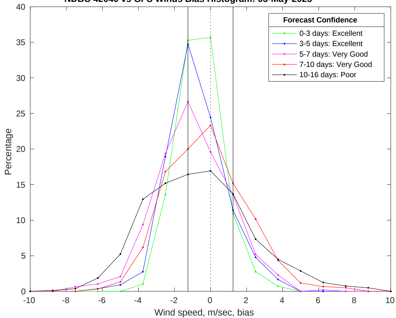
NDBC 42040 vs GFS Winds Bias Histogram: 03-May-2025
