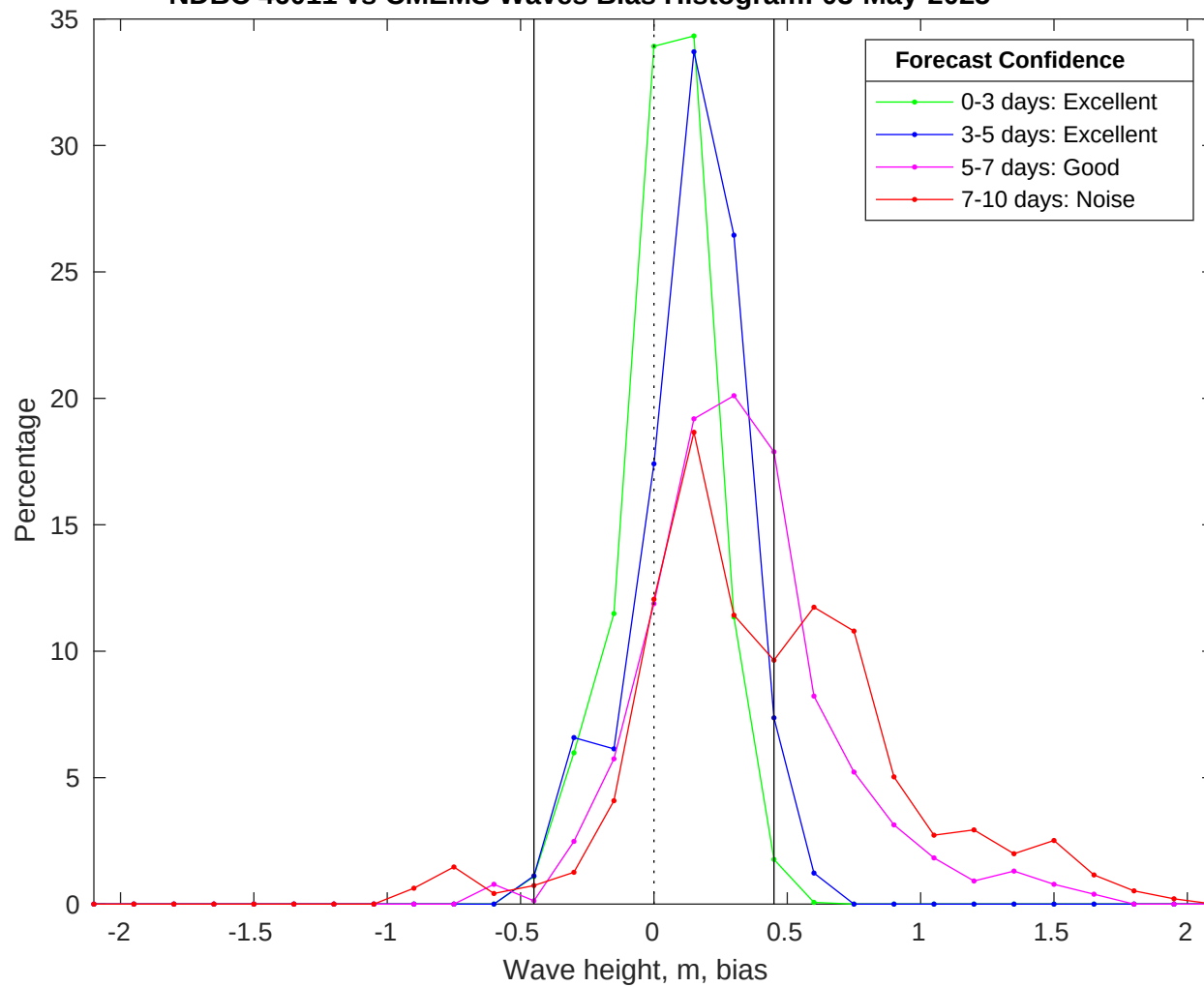
NDBC 46011 vs CMEMS Waves Bias Histogram: 03-May-2025
