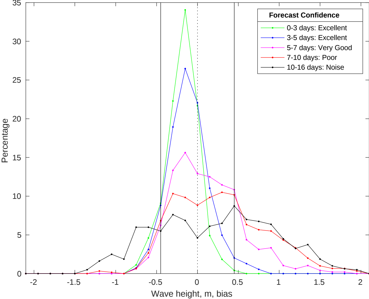
NDBC 46011 vs GFS Waves Bias Histogram: 03-May-2025
