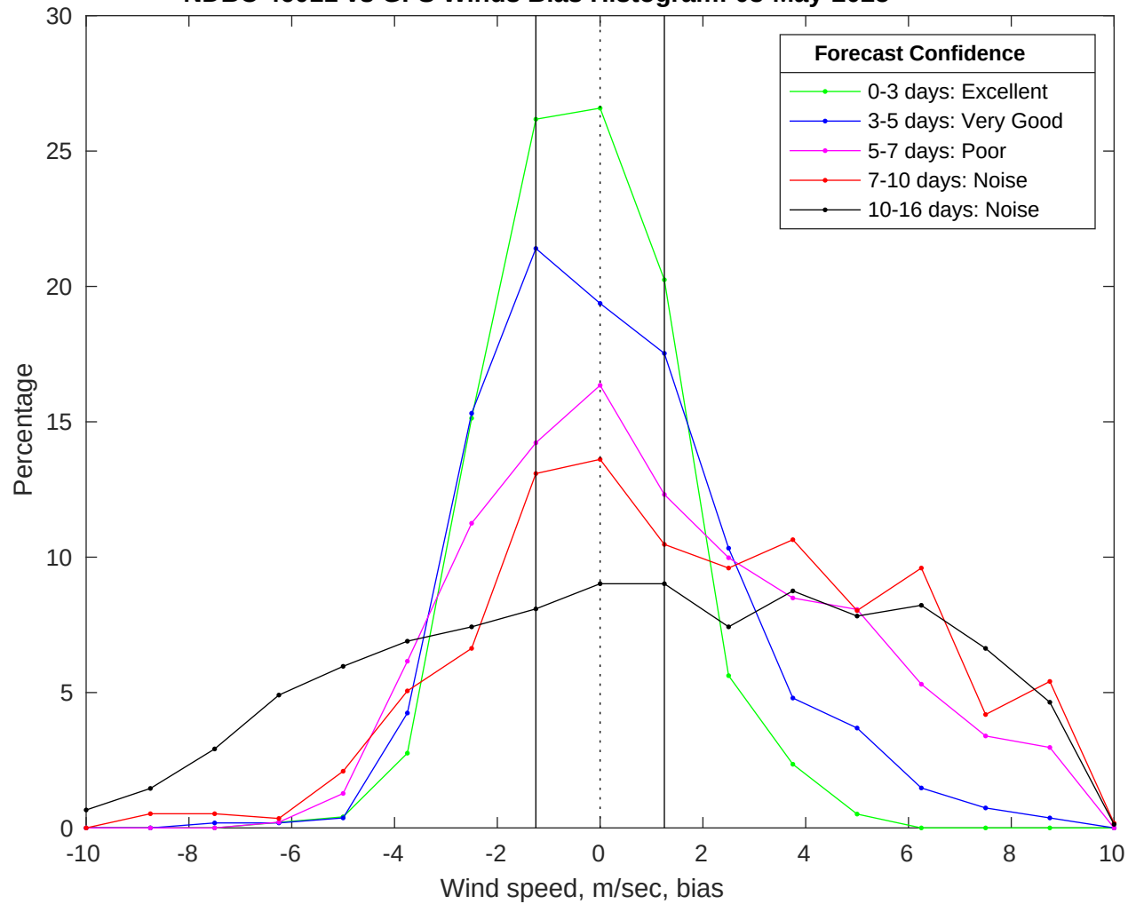
NDBC 46011 vs GFS Winds Bias Histogram: 03-May-2025
