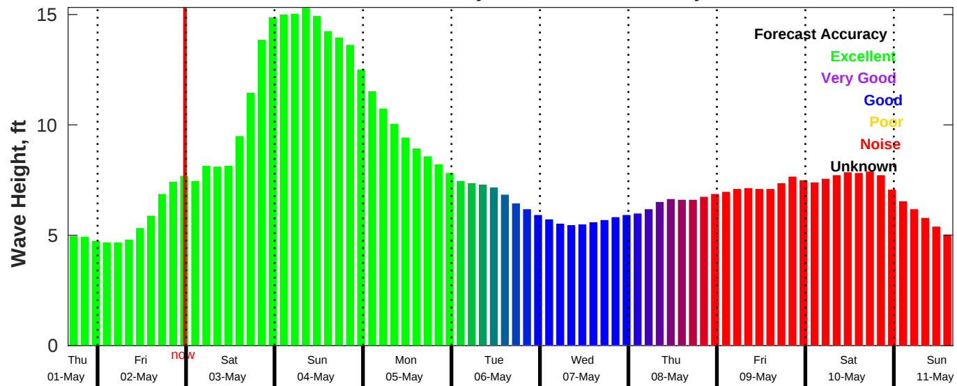
CMEMS Wave Forecast for NDBC 46011 from 01-May-2025 16:00:00 to 11-May-2025 16:00:00
