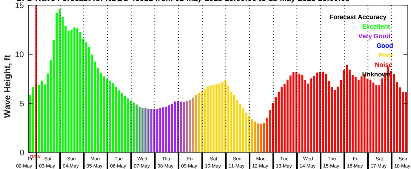
GFS Wave Forecast for NDBC 46011 from 02-May-2025 16:00:00 to 18-May-2025 16:00:00
