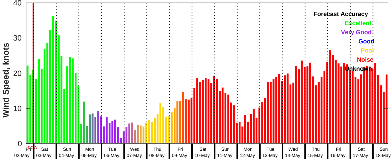
GFS Wind Speed Forecast for NDBC 46011 from 02-May-2025 16:00:00 to 18-May-2025 16:00:00
