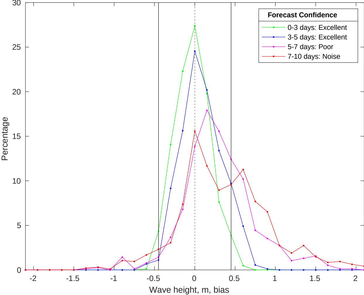
NDBC 46028 vs CMEMS Waves Bias Histogram: 03-May-2025
