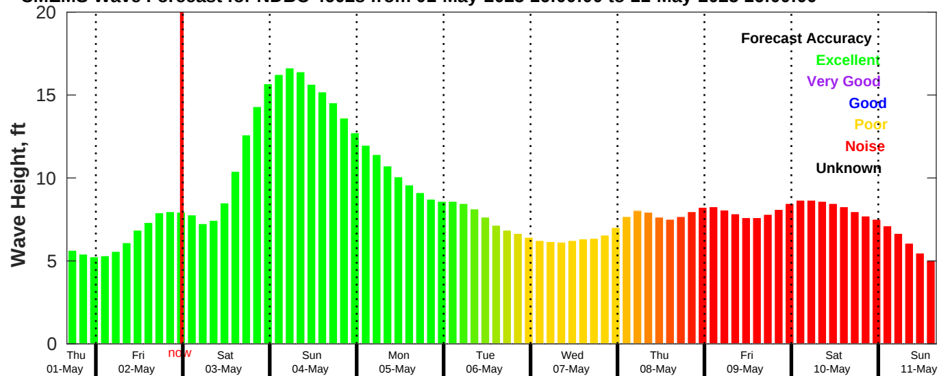
CMEMS Wave Forecast for NDBC 46028 from 01-May-2025 16:00:00 to 11-May-2025 16:00:00
