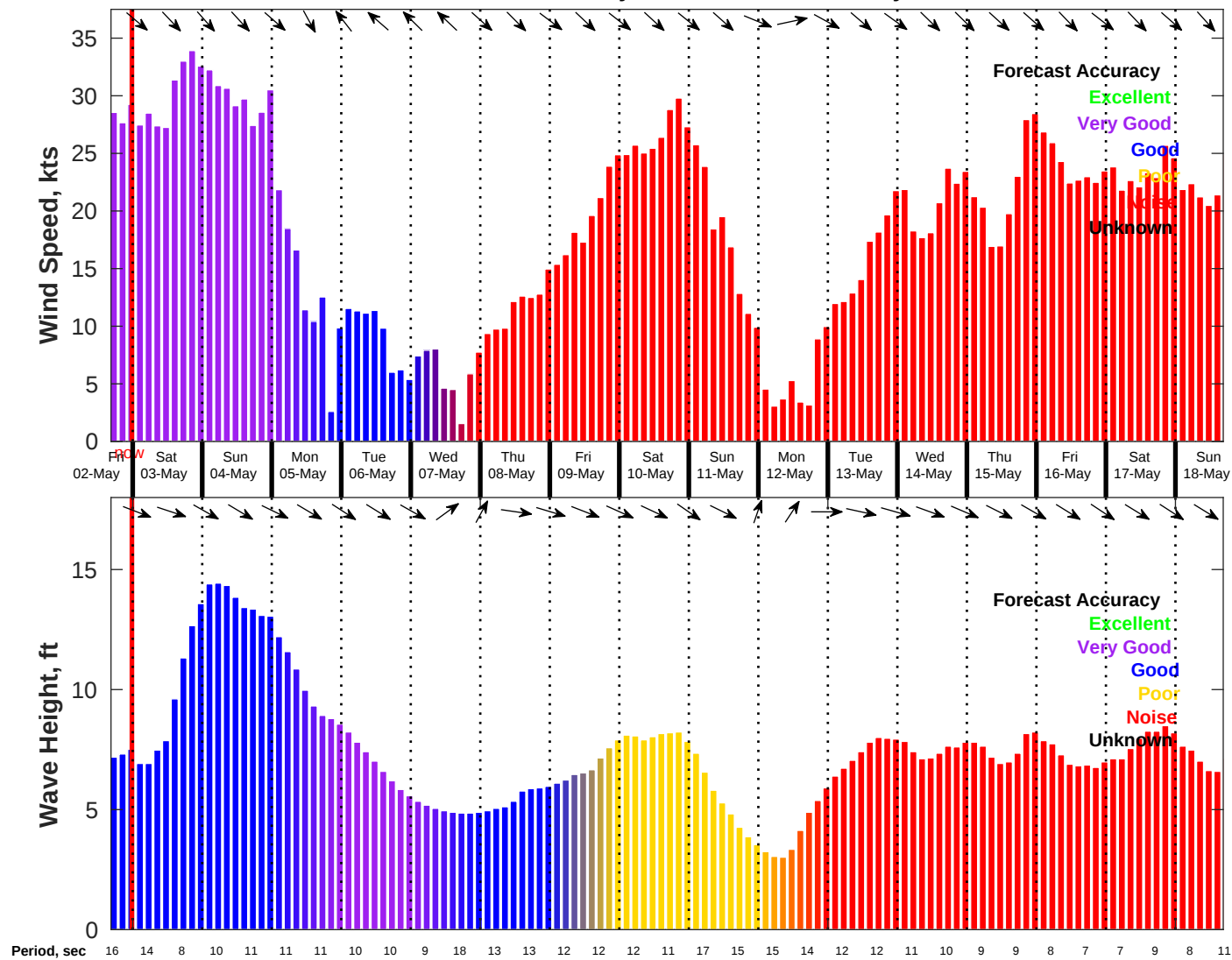
Wind & Wave Forecast for NDBC 46028 from 02-May-2025 16:00:00 to 18-May-2025 16:00:00
