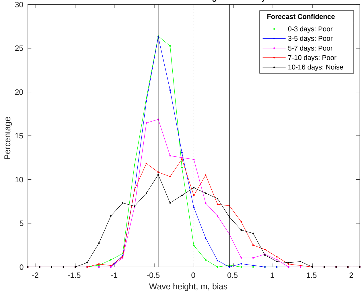
NDBC 46054 vs GFS Waves Bias Histogram: 03-May-2025
