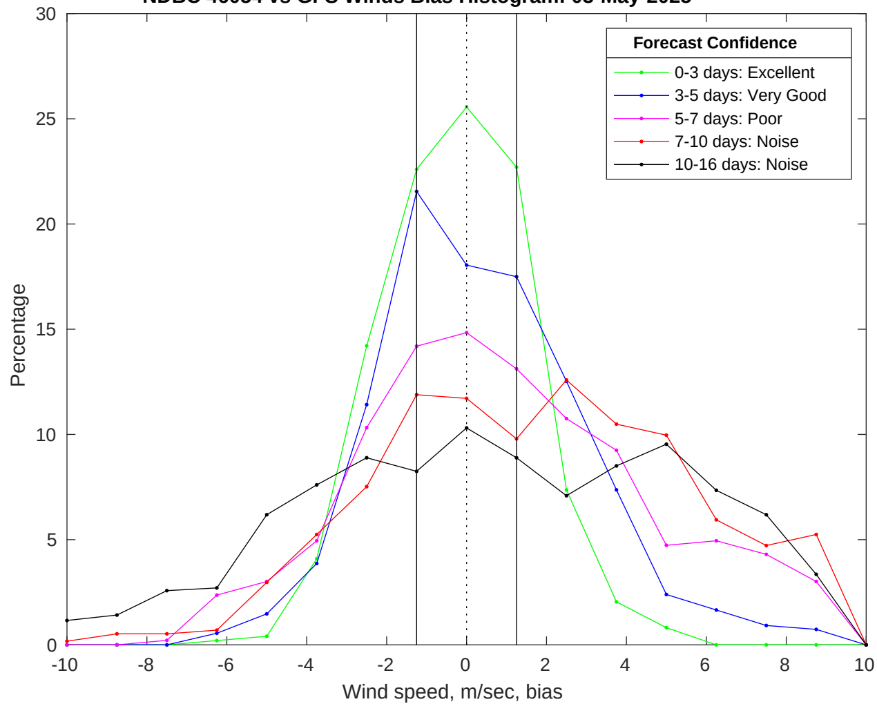
NDBC 46054 vs GFS Winds Bias Histogram: 03-May-2025
