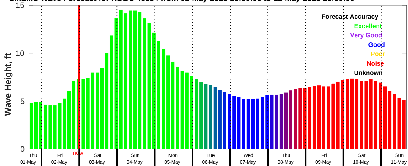
CMEMS Wave Forecast for NDBC 46054 from 01-May-2025 16:00:00 to 11-May-2025 16:00:00
