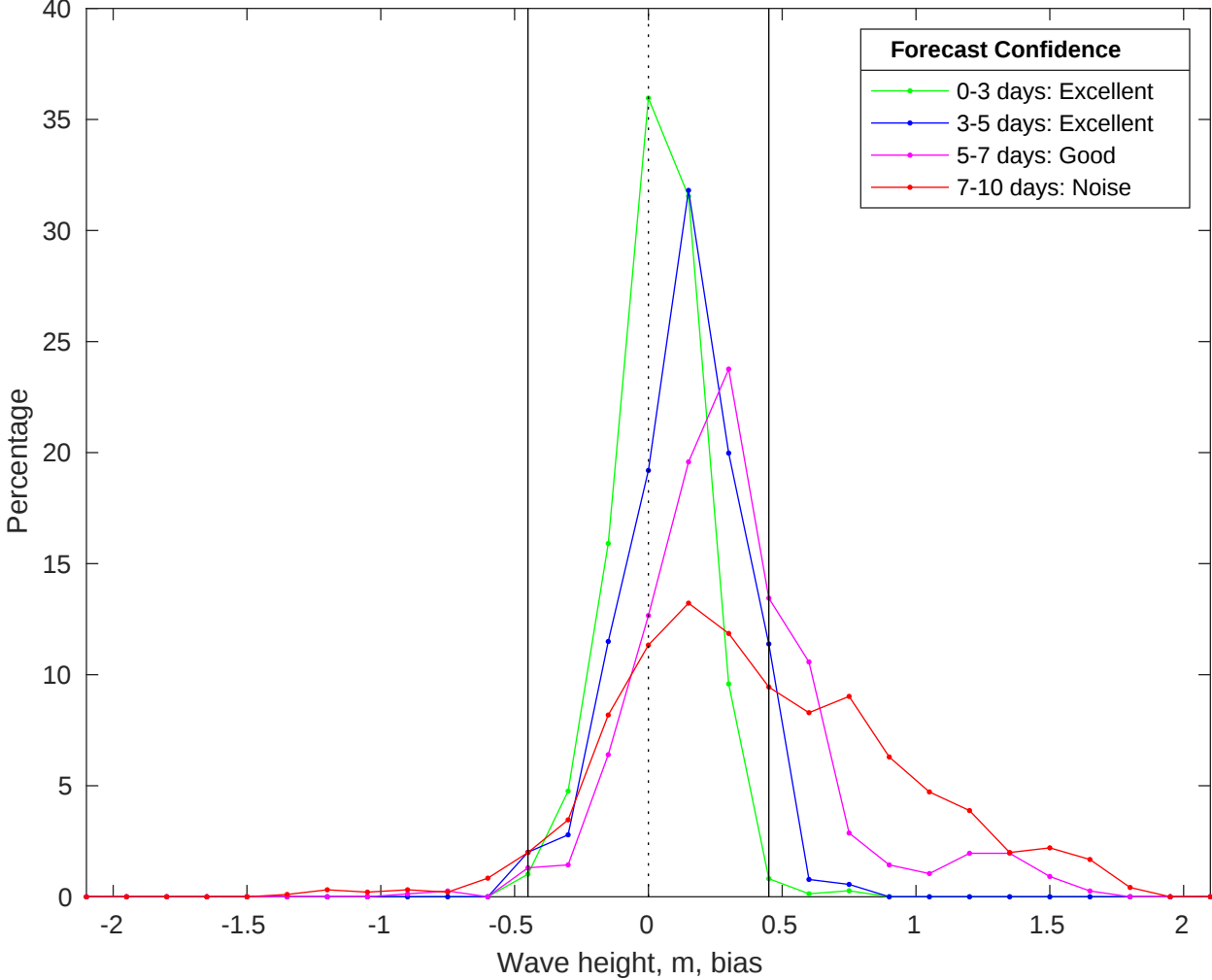
NDBC 46069 vs CMEMS Waves Bias Histogram: 03-May-2025
