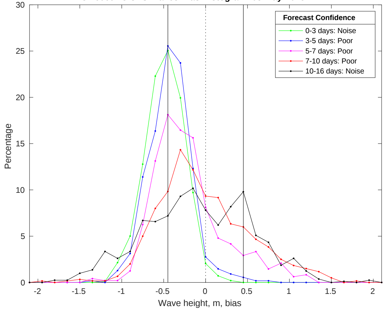
NDBC 46069 vs GFS Waves Bias Histogram: 03-May-2025
