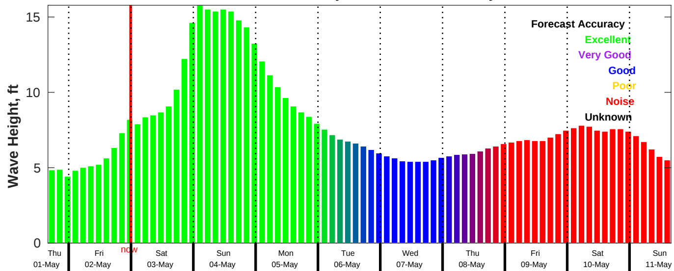
CMEMS Wave Forecast for NDBC 46069 from 01-May-2025 16:00:00 to 11-May-2025 16:00:00
