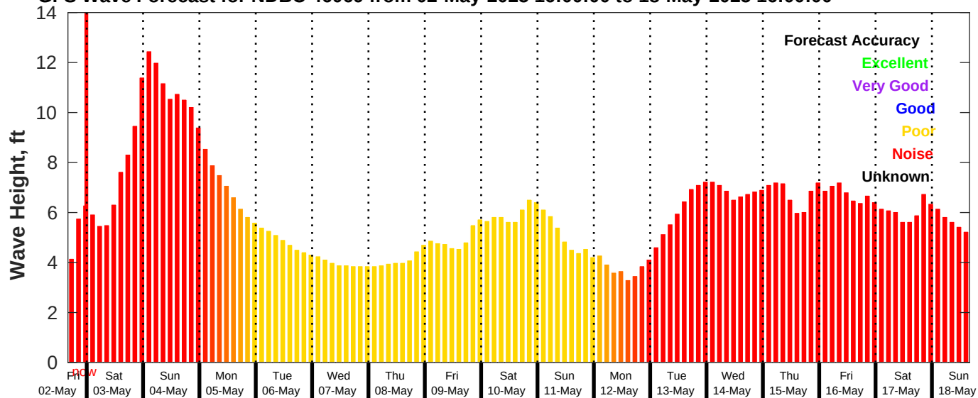
GFS Wave Forecast for NDBC 46069 from 02-May-2025 16:00:00 to 18-May-2025 16:00:00
