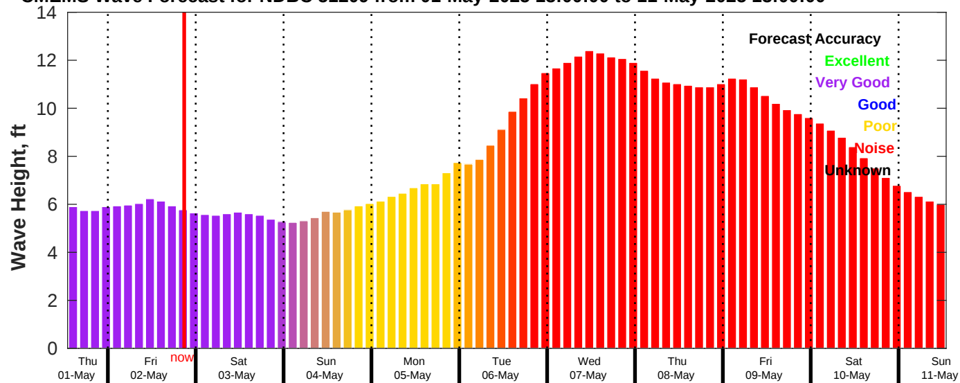
CMEMS Wave Forecast for NDBC 51209 from 01-May-2025 13:00:00 to 11-May-2025 13:00:00
